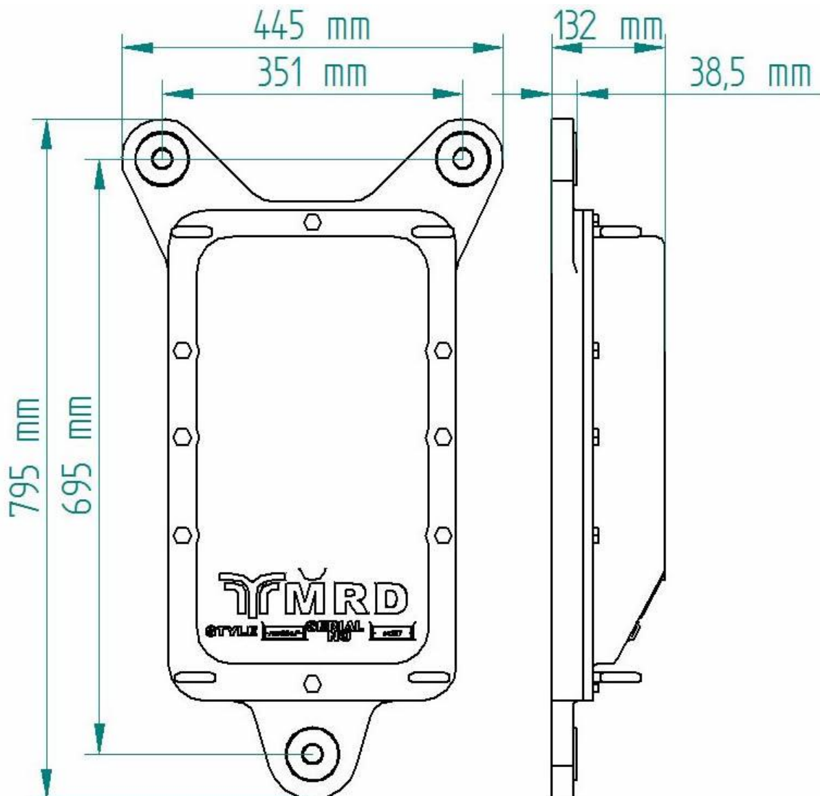
Figure 3 – Dimensions of the AWS 1 – LP.
